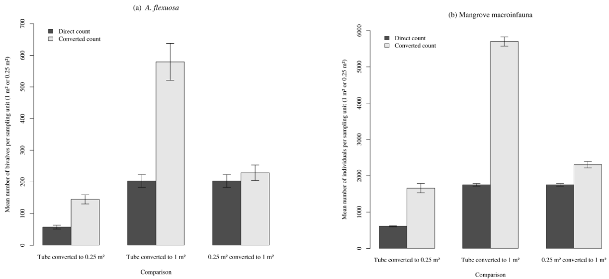
Figure 1. Mean values ± s.e. (n=60) of direct and converted (from a 0.007854 m 2 tube and 0.25 m 2 quadrat) counts of (a) Anomalocardia flexuosa and (b) mangrove macroinfauna in 0.25 m 2 and 1 m 2 quadrats.
