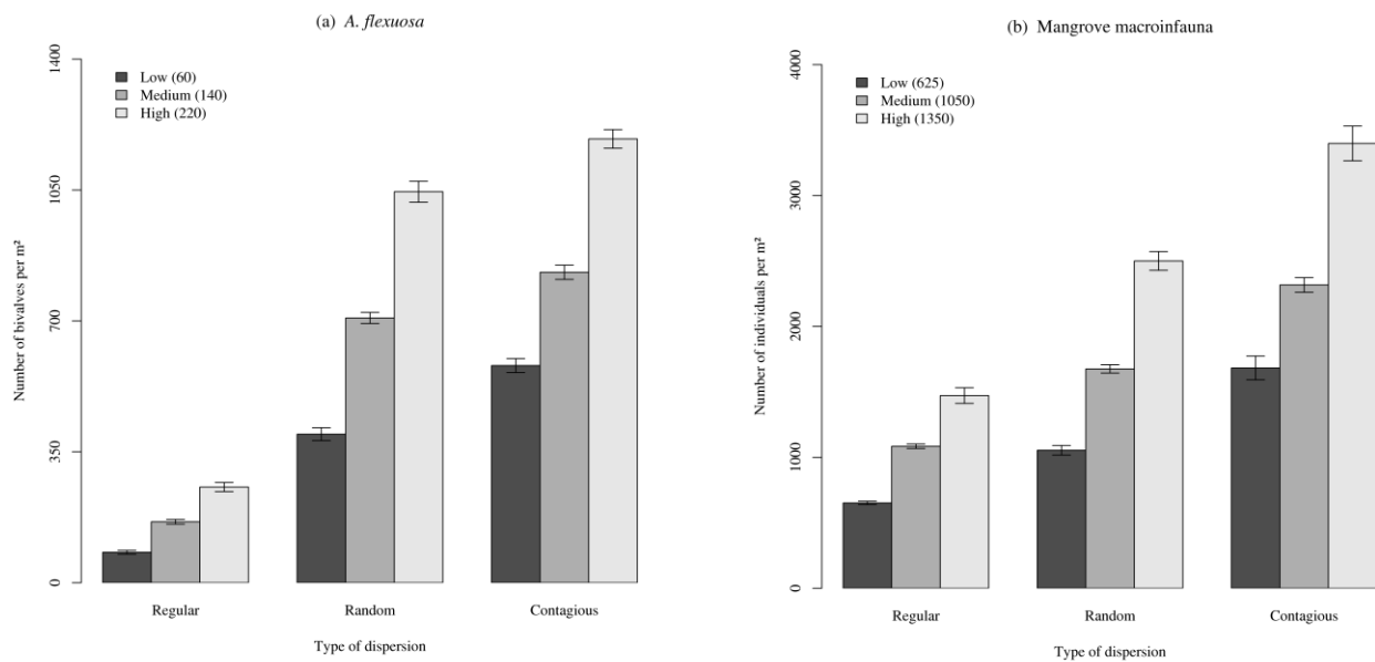
Figure 2. Mean ( \pm s.e.) converted counts of (a) Anomalocardia flexuosa and (b) objects representing mangrove macroinfauna in 1 m 2 quadrats at low, medium and high densities and with regular, random and contagious dispersion. The direct counts (in 1 m 2 ) for each faunal group is indicated in the respective figure legends.
