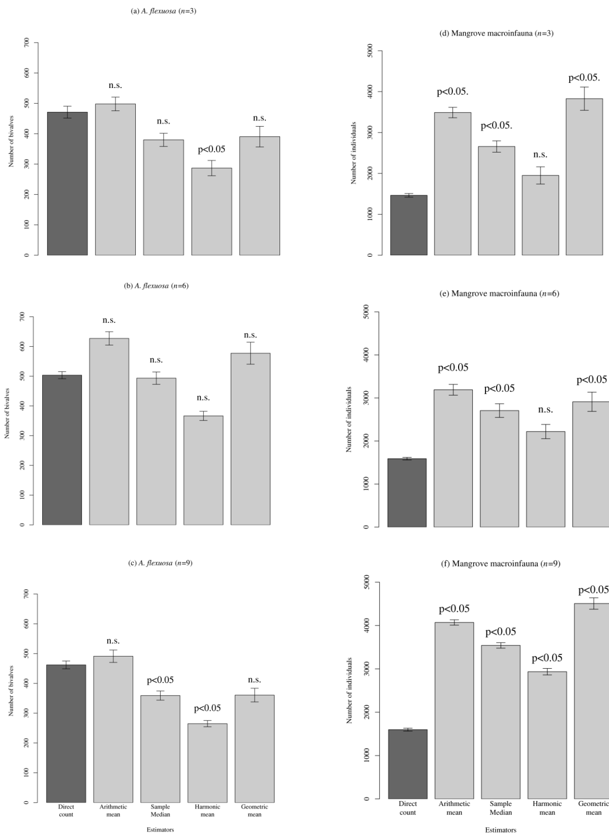
Figure 3. Comparison of mean ( \pm s.e.) direct (dark gray) and converted (light gray) counts, using the arithmetic mean, sample median, geometric mean and harmonic mean, of (a,b,c) Anomalocardia flexuosa and (d,e,f) mangrove macroinfauna in samples of n=3 , 6 and 9 replicas, respectively, in 1 m 2 quadrats. The significance (p) of Dunnet's test for the comparison of the direct count with each converted count, is given above the bar.
